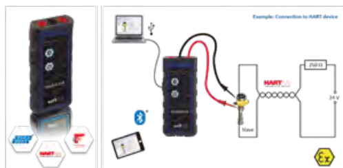
Interface Multiprotocolo MobiLink
